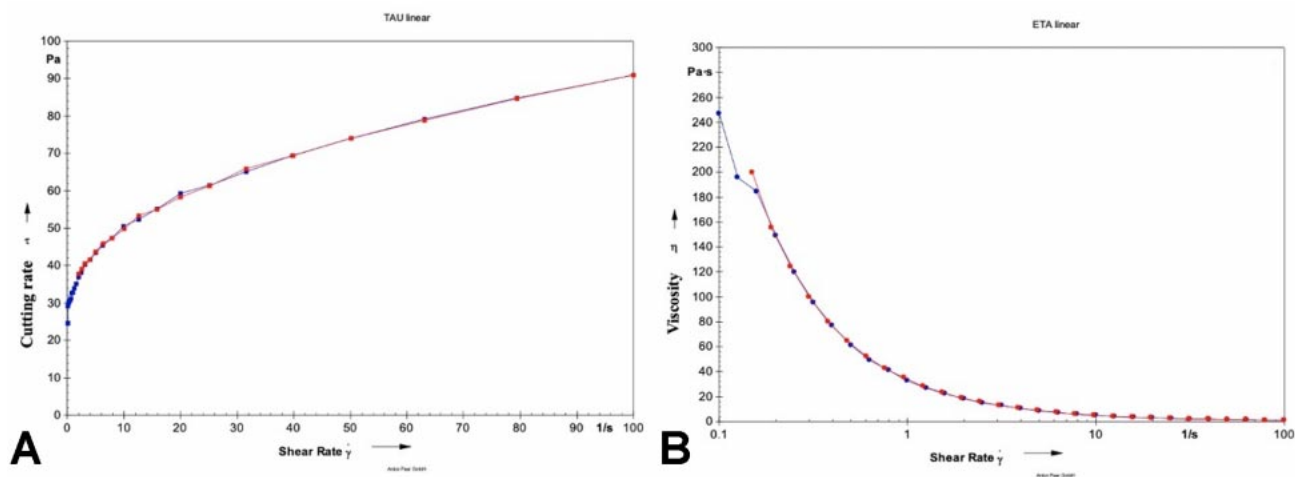
Fig. 3. Hydrogel characteristics. a) Hydrogel flow curve, b) Hydrogel viscosity curve.
